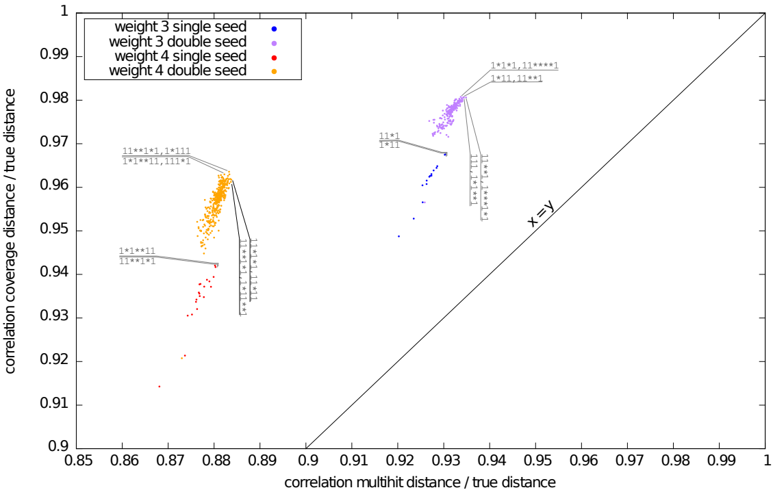
True distance Correlation with MultiHit (x) vs Coverage (y) distance
